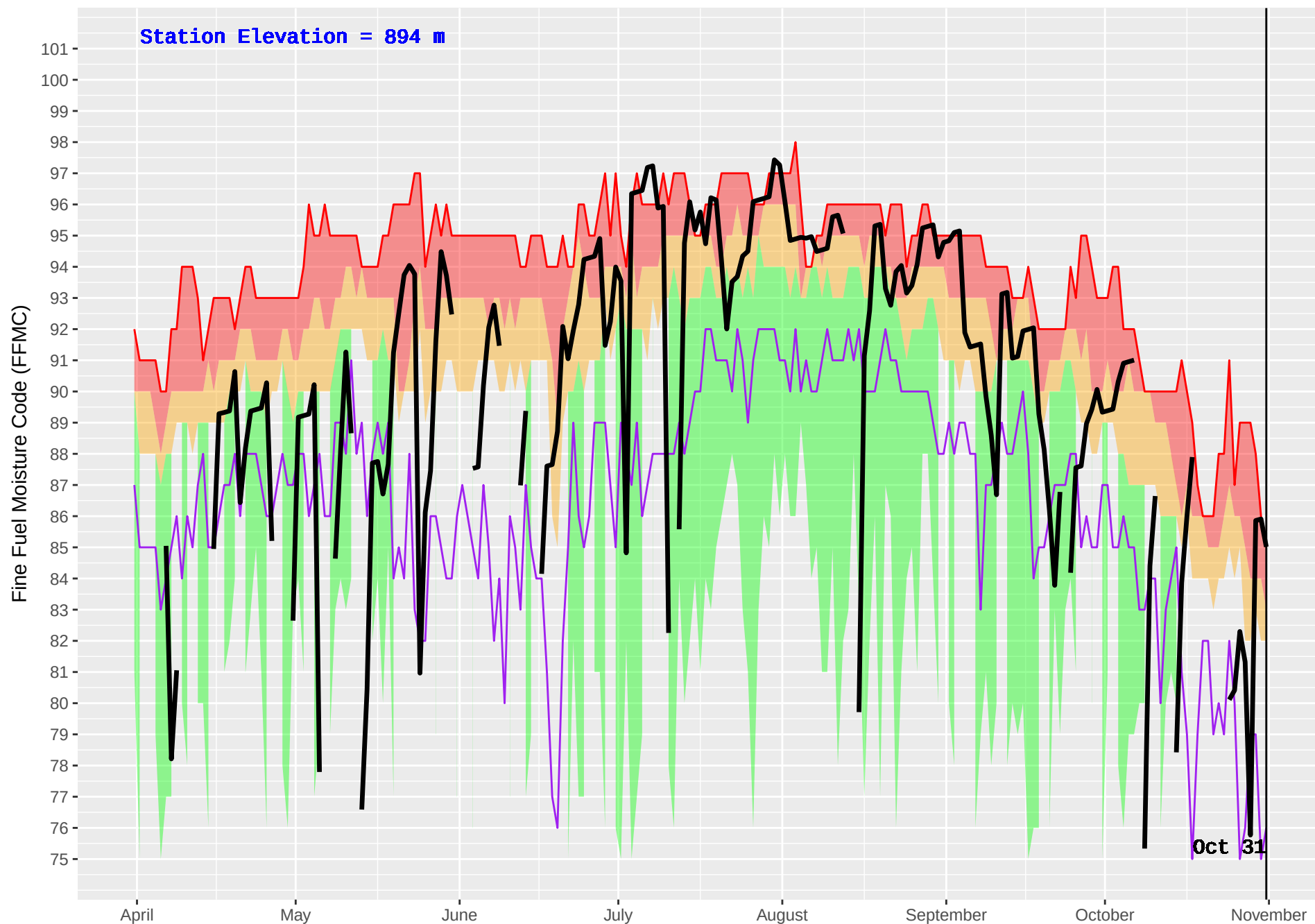
TOBY HUB (417) : Historical (1986–2016) and Current (2017) Noon Fine Fuel Moisture Code (FFMC)
